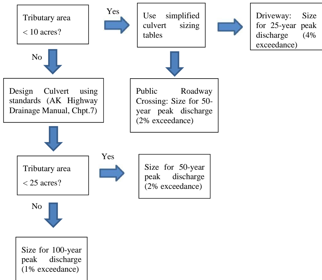
Figure 1. Determination of Design Flows
